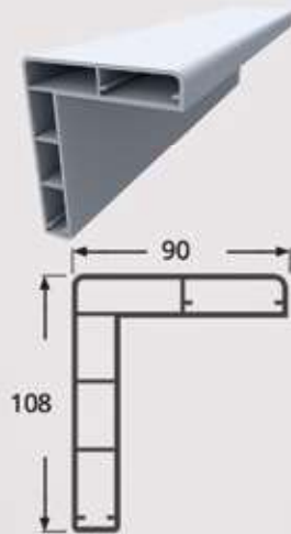
Back Cover PVC Profile
