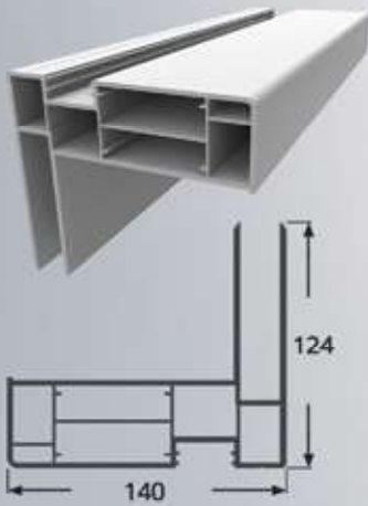
Main Part PVC Profile
