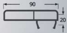
Back Cover PVC Profile
