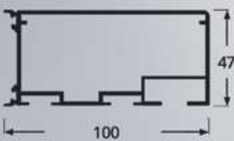
Main Part Aluminium Profile
